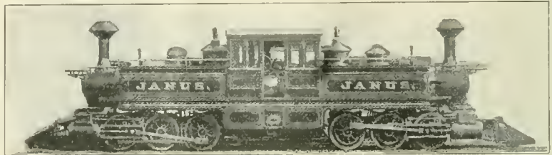
MASON'S DOUBLE END LOCOMOTIVE. FIG. 53.
